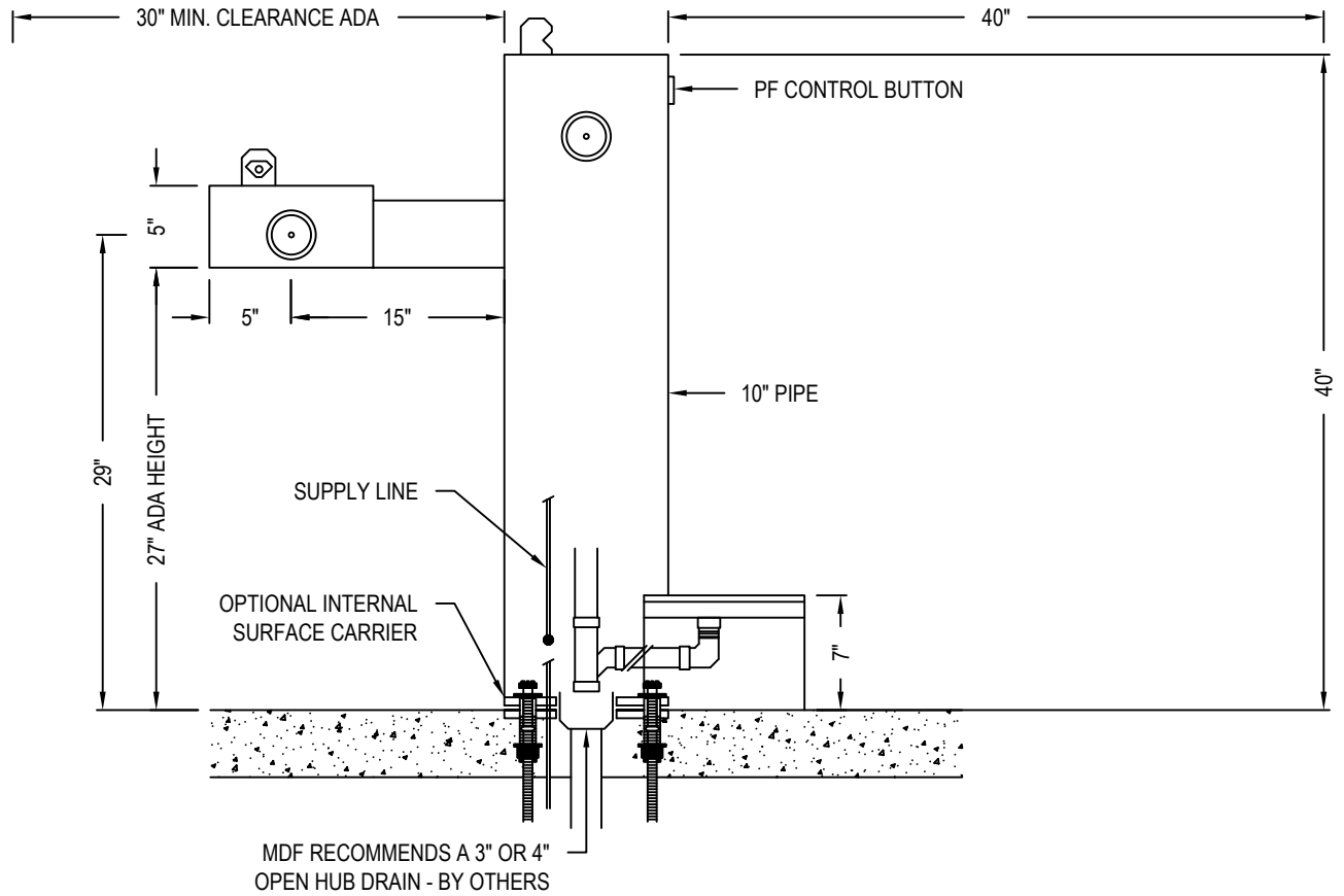
FRONT VIEW
